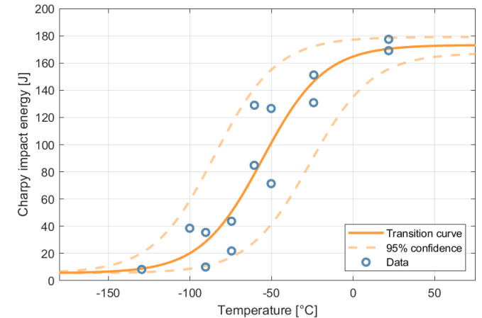
The ductile to brittle transition curve of the impact toughness test results from the RPV head mase material.
