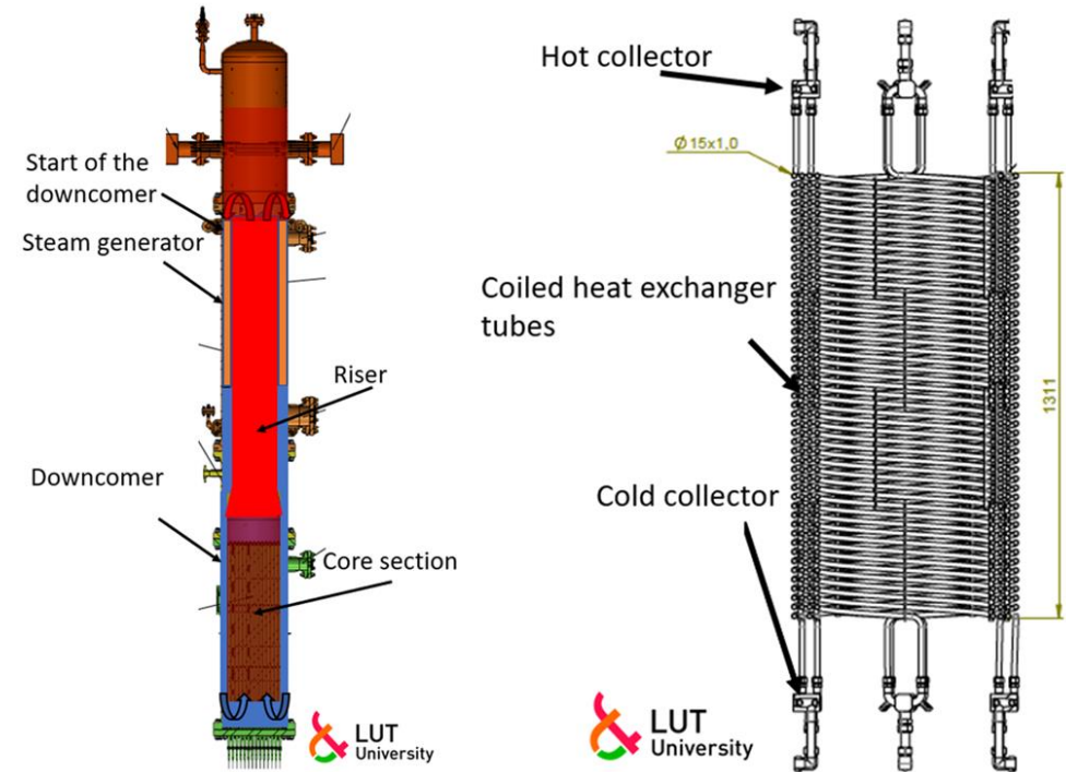
Water flow paths in the primary side and steam generator tubes and collectors of the MOTEL facility.
